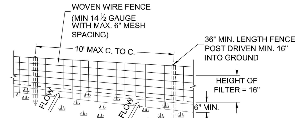
PERSPECTIVE VIEW
